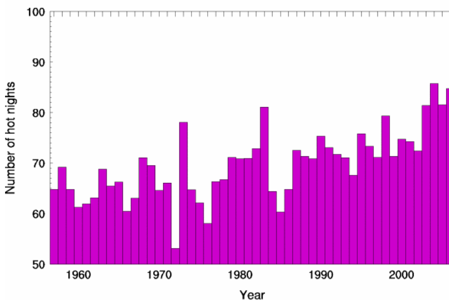
Figure 2: Average number of hot nights in Australia over 30 years
