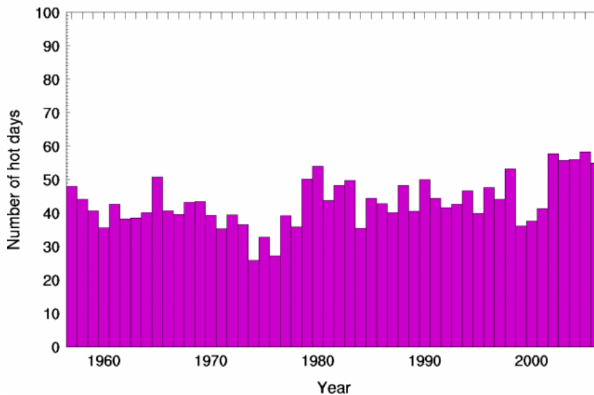
Figure 1: Average number of hot days in Australia over 30 years
