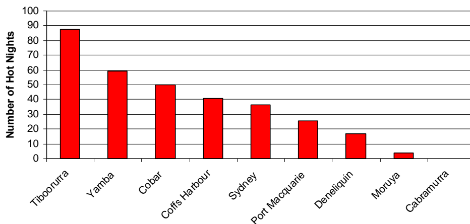
Figure 4: Average number of hot nights across NSW (1962–2006)
